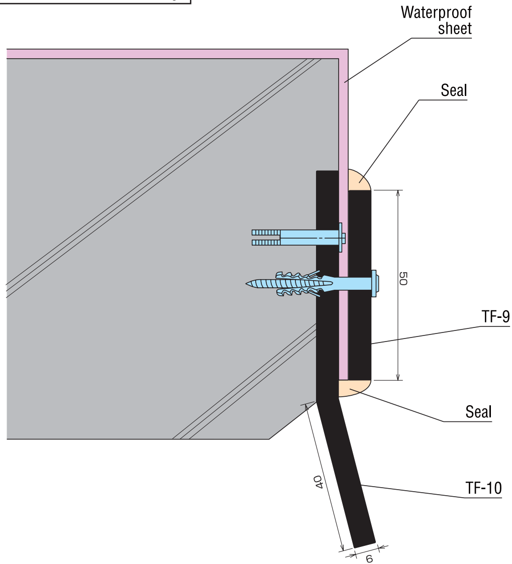
TA-9, 10 Installation drawings
